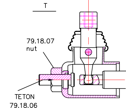
P80 directional control valve
